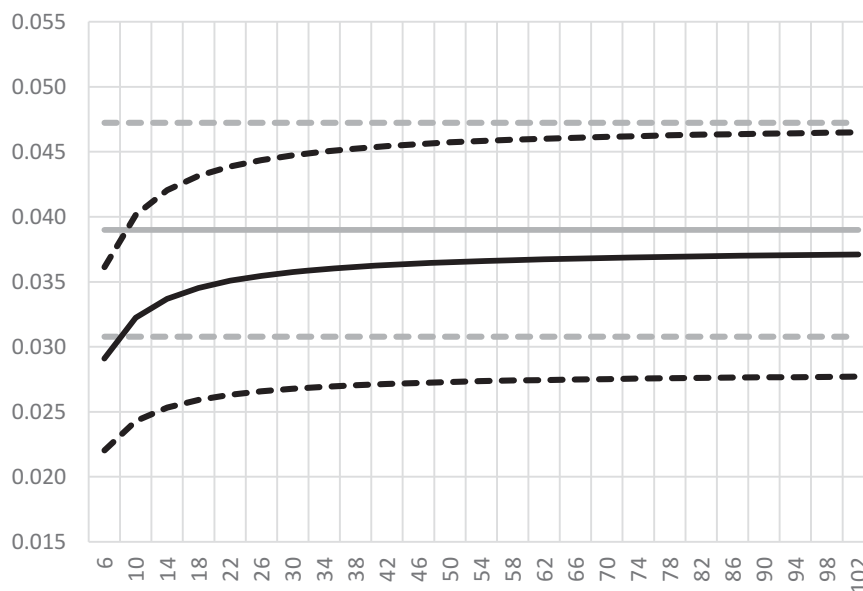
FIGURE A1 Estimated coefficients on VIX of censored Poisson vs. PPML for different months assigned to non-granted loans
