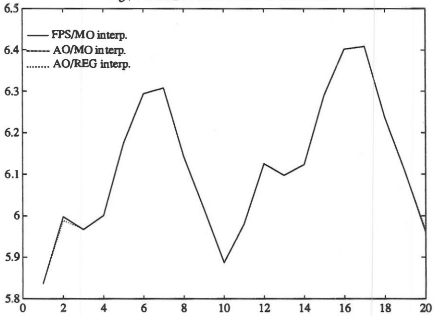
Fig.7 : THREE INTERPOLATION METHODS
