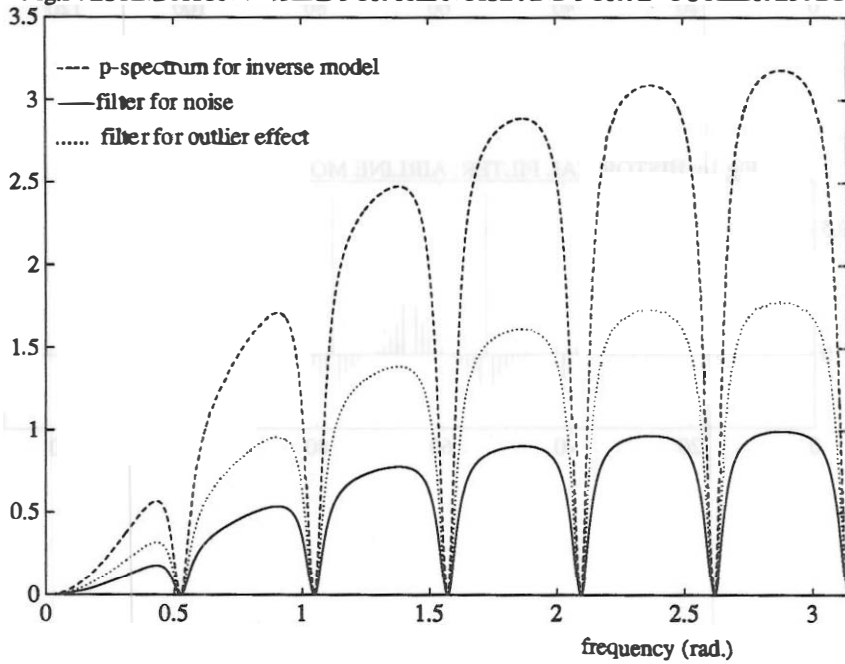
Fig.3 : ESTIMATION FILTERS FOR THE NOISE AND FOR AN OUTLIER EFFECT
