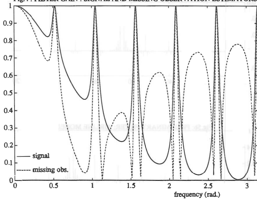
Fig.4 : FILTER GAIN : SIGNAL AND MISSING OBSERVATION ESTIMATORS
