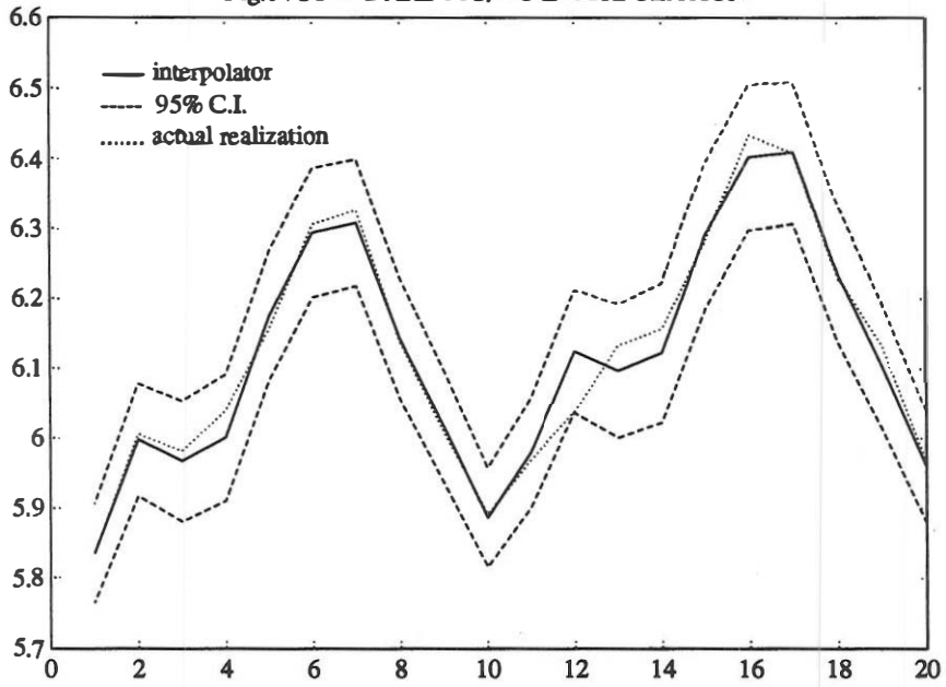
Fig.6 : STANDARD FPS/MO INTERPOLATION
