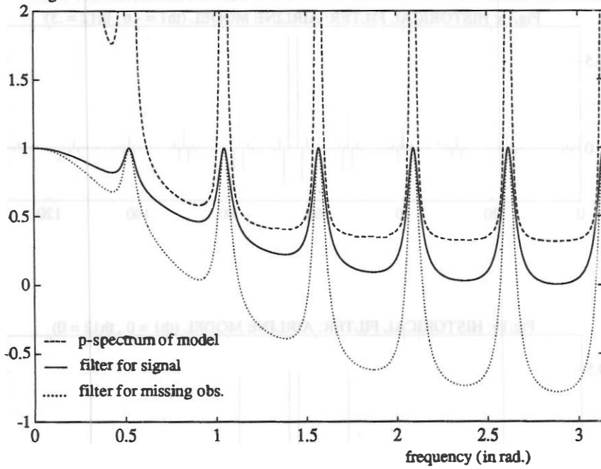
Fig.2 : ESTIMATION FILTERS FOR THE SIGNAL AND FOR A MISSING OBS.
